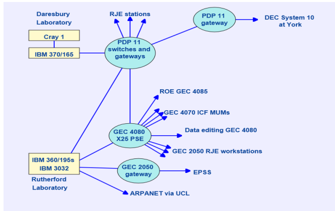
Figure 12 SERCNET Topology (1977)
