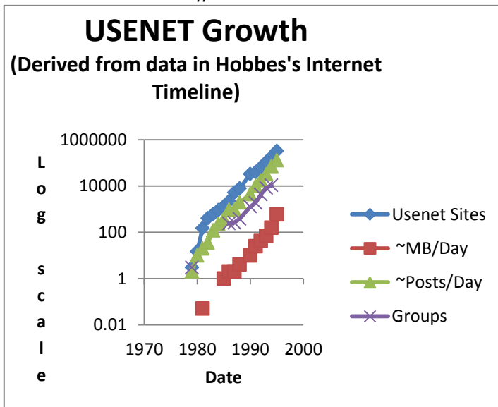
Figure 6 USENET Growth
